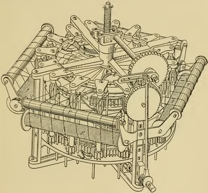
CIRCULAR LOOM.
